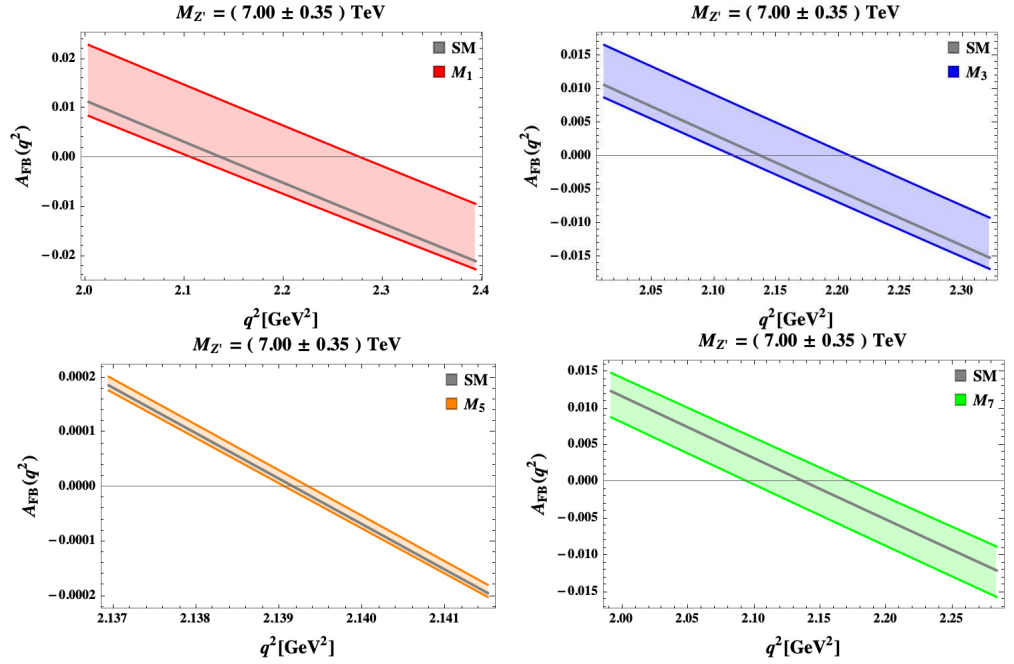
Figure 7. Zoom of the region close to the zero of the forward-backward asymmetry (49) for B \rightarrow K^* \mu^+ \mu^- . The SM prediction is compared to M_1 (top-left), M_3 (top-right), M_5 (bottom-left) and M_7 (bottom-right) in the case M_{Z'} \simeq 7 TeV. Same legend as in Figure 4.
