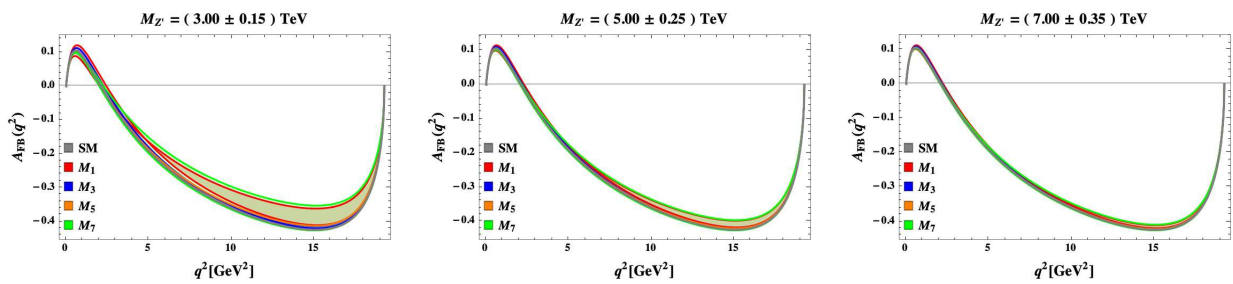
Figure 4. Forward-backward asymmetry (49). The SM prediction (gray curve) is compared to the four considered 331 models and M_{Z'} \simeq 3 TeV (left), M_{Z'} \simeq 5 TeV (middle) and M_{Z'} \simeq 7 TeV (right panel). For M_i models, the legend is the same as in Figure 3.
