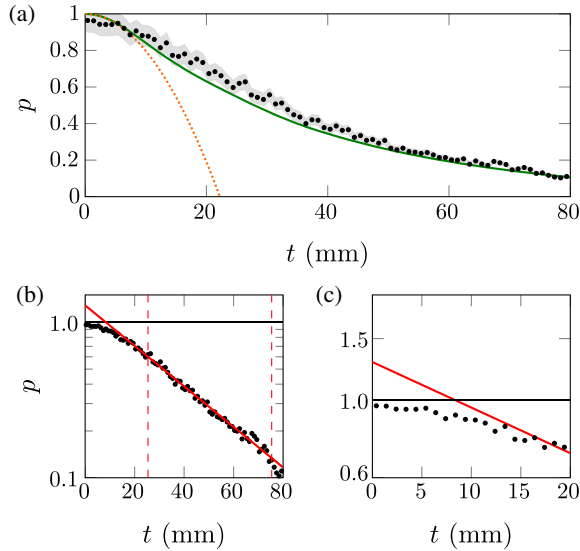
FIG. 2. Experimental survival probability in a weakly coupled system (array A in Table I). Experimental points (black dots) are reported in linear (a) and semilogarithmic plots (b),(c). Experimental errors are shown in the linear plot as a gray area around the points. The green continuous line in (a) is the theoretical prediction, obtained by solving Eq. (5) with the nominal data ( \kappa_0 , \kappa , \varepsilon , q ) of array A . The orange dotted line in (a) is the parabolic trend 1 - (t/\tau_z)^2 with \tau_z = 1/\kappa_0 . The red continuous line in (b) and (c) is a linear fit performed on the semilogarithmic plot, considering the data between the two dashed red lines in (b).
