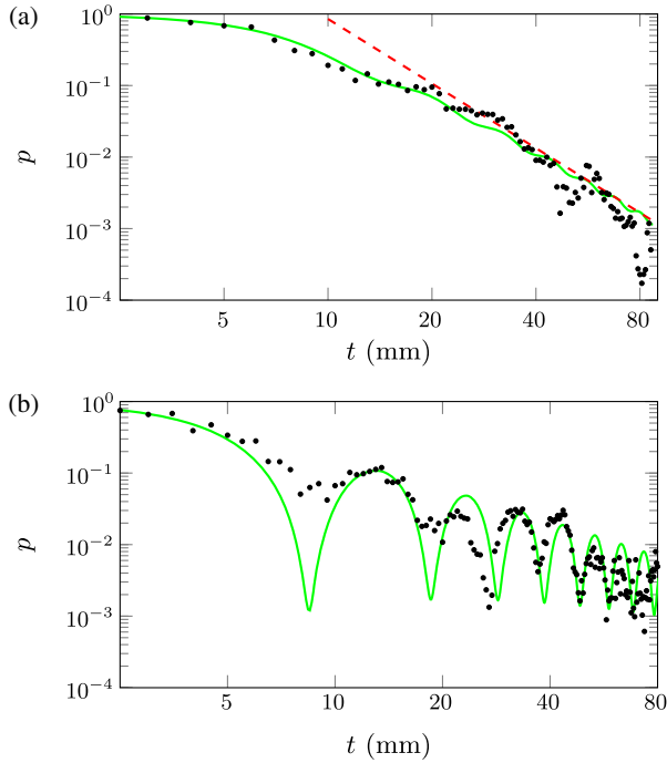
FIG. 3. Experimental survival probability in systems with stronger coupling, i.e., array B [(a)] and array C [(b)] in Table I. Experimental points (black dots) are reported in logarithmic plots; experimental errors are comparable to the marker size. The (green) solid lines represent data fitting, obtained by solving Eq. (5) using (a) \kappa_0 = 0.119 \text{ mm}^{-1} , \kappa = 0.132 \text{ mm}^{-1} , \varepsilon = 0.12 \text{ mm}^{-1} , and q = 0.01 \text{ mm}^{-1} and (b) \kappa_0 = 0.205 \text{ mm}^{-1} , \kappa = 0.160 \text{ mm}^{-1} , \varepsilon = 0 \text{ mm}^{-1} , and q = 0.01 \text{ mm}^{-1} ; the fitting parameters are close to the nominal ones reported in Table I. The (red) dashed line in (a) represents the polynomial trend p(t) \simeq (C_\infty/t)^3 .
