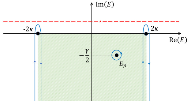
FIG. 1. Representation of the integration paths used to obtain the survival amplitude from its Fourier-Laplace transform G(E) . The (red) dashed line above the real axis represents the integration path in Eq. (6), that can be deformed into the (blue) solid path, composed of three separate curves. Part of the new path lies on the second Riemann sheet of the propagator (shaded area), where G(E) has been analytically continued from above across the cut singularity in [-2\kappa, 2\kappa] . The imaginary part of the pole E_p determines the decay rate \gamma .
