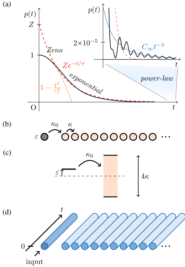
FIG. 1. (a) Typical decay of a quantum state coupled to a continuum, showing the peculiar features of the survival probability p(t) . The initial region is quadratic, with the curvature at t = 0 characterized by the Zeno time \tau_Z . At intermediate times, a familiar exponential decay sets in, with a lifetime \tau = O(\lambda^{-2}) , where \lambda is the coupling constant, and a “wave-function renormalization” Z = 1 + O(\lambda^2) , which represents the value of its extrapolation back to t = 0 . At very large times, when the survival probability is reduced to O(\lambda^{10}) , a power-law regime is observed, with superimposed oscillations. In particular, we refer to the system represented in (b): An optical mode with detuning \varepsilon is coupled, by a coupling constant \kappa_0 , to a chain of optical modes with relative coupling \kappa . (c) Level scheme of such a system: The states of the chain make up a continuum with bandwidth 4\kappa (as in a tight-binding one-dimensional lattice). (d) Experimentally, we study this system with an array of single-mode optical waveguides.
