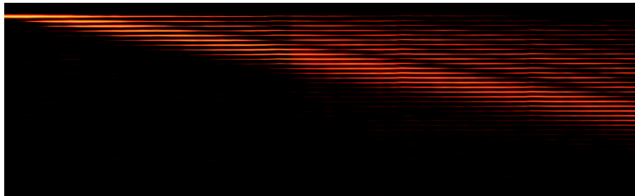
FIG. 3. Example of acquired intensity distribution from a waveguide array (array B in Table 1 of the Main Text). Laser light is coupled in the array from the left in the topmost waveguide. The original acquisition is monochrome and measures 89 (horizontal) \times 1280 (vertical) pixels (corresponding to a physical region of about 88 \text{ mm} \times 640 \mu\text{m} sampled longitudinally with steps of 0.5 \text{ mm} ). Here the image is reshaped for better readability and is shown using a logarithmic false-color scale. Note that the last illuminated waveguide is the 30^{\text{th}} (counting from top) of the 40 -waveguide array. In this condition the semi-infinite model is valid.
