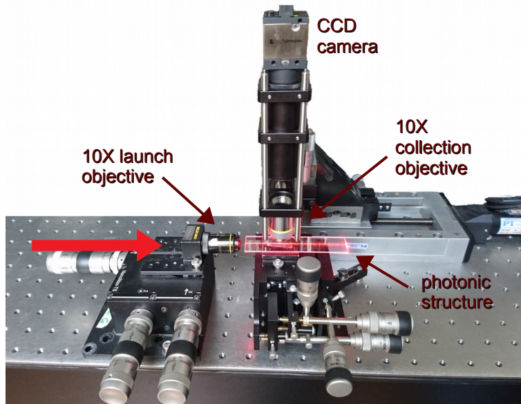
FIG. 2. Picture of the experimental apparatus employed to characterize the light distribution along propagation, in the fabricated waveguide arrays.
